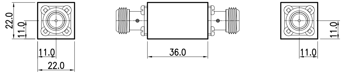
(2) N TYPE
