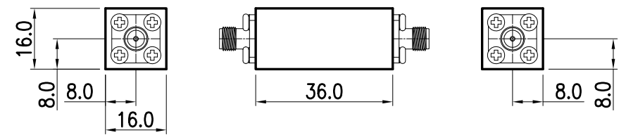
(1) SMA TYPE
